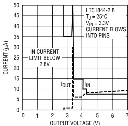
Figure 7. Reverse Current vs Output Voltage
