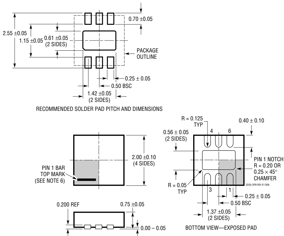
DC Package 6-Lead Plastic DFN (2mm × 2mm) (Reference LTC DWG # 05-08-1703 Rev B)
