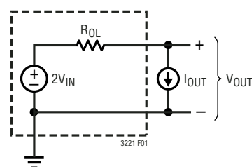
Figure 1. Equivalent Open-Loop Circuit
