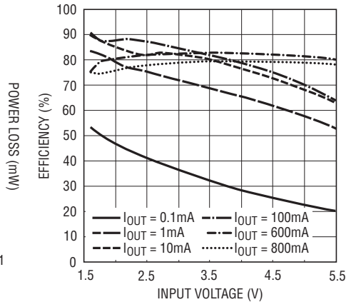
Efficiency vs Input Voltage V_{OUT} = 1.2V , Burst Mode Operation
