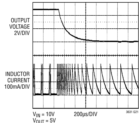
Short-Circuit Response
