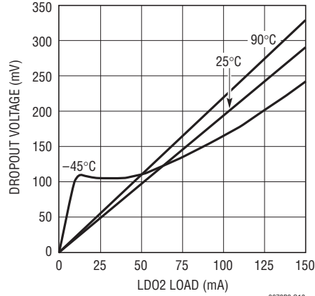
V_{IN} – LD02 Dropout Voltage vs Load
