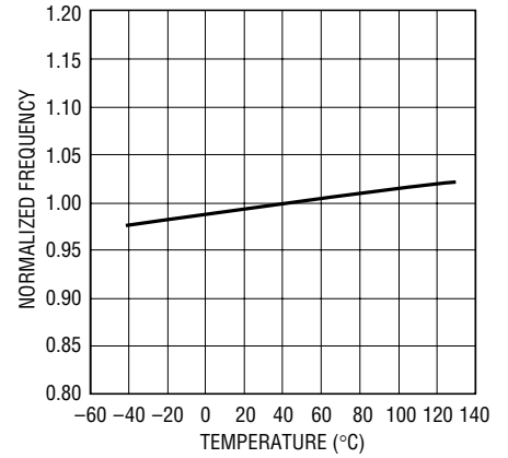
Normalized Frequency vs Temperature
