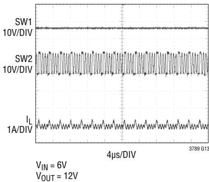
Pulse-Skipping Mode
