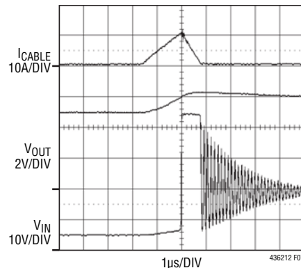
R_{IN} = 150\text{m}\Omega , L_{IN} = 2\mu\text{H} LOAD = 10\Omega C_{OUT} = 10\mu\text{F} (16V, SIZE 1210)
