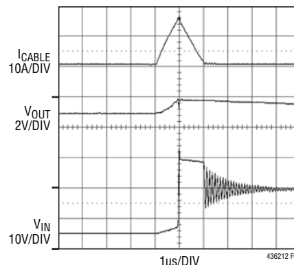
R_{IN} = 150\text{m}\Omega , L_{IN} = 0.7\mu\text{H} LOAD = 10\Omega C_{OUT} = 10\mu\text{F} (16V, SIZE 1210)
