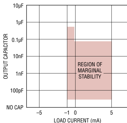
1.25V Stability with Output Capacitance
