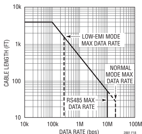
Figure 18. Cable Length vs Data Rate
