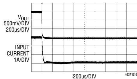
Short-Circuit Protection with 20A Load
