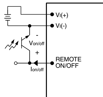
Figure 38. Remote On/Off Implementation
