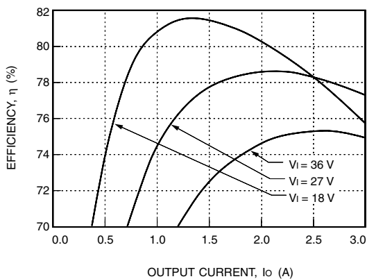
Figure 18. LC015F Typical Efficiency vs. Output Current at T_c = 25\text{ }^\circ\text{C}
