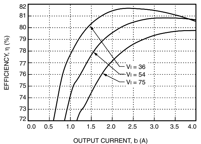
Figure 5. LW020A Typical Converter Efficiency vs. Output Current
