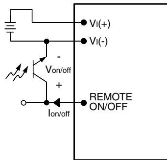
Figure 14. Remote On/Off Implementation
