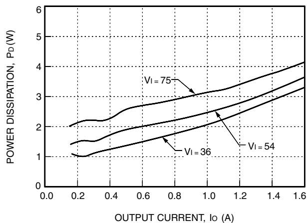
Figure 19. LW020B Power Dissipation vs. Output Current, T_A = 25\text{ }^{\circ}\text{C}
