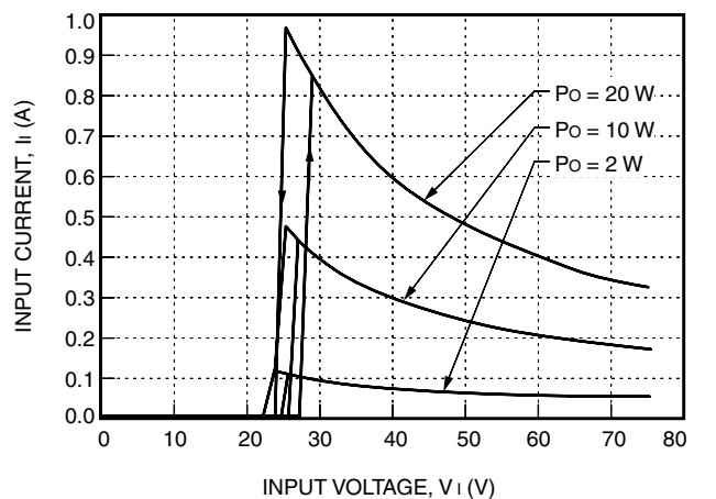
Figure 1. LW020 Typical Input Characteristics, T_A = 25\text{ }^{\circ}\text{C}
