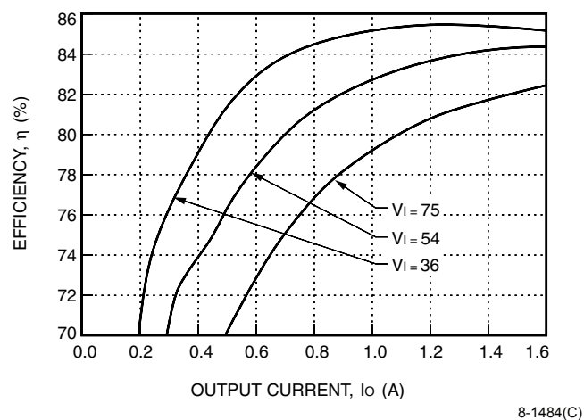
Figure 6. LW020B Typical Converter Efficiency vs. Output Current, T_A = 25^\circ\text{C}
