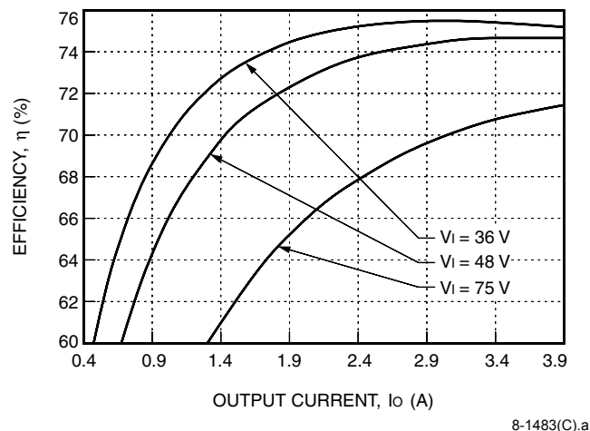
Figure 3. LW020G Typical Converter Efficiency vs. Output Current, T_A = 25\text{ }^{\circ}\text{C}
