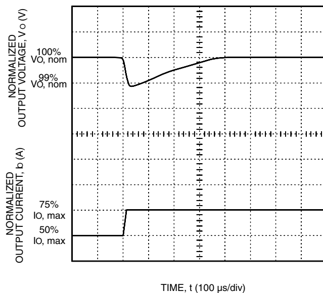
Figure 8. LW020A, B, C, F, and G Typical Output Voltage for a Step Load Change from 50% to 75%
