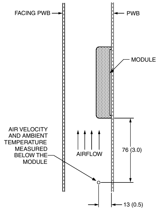
Figure 21. Experimental Test Setup
