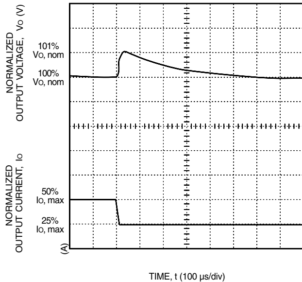
Figure 9. LW020A, B, C, F, and G Typical Output Voltage for a Step Load Change from 50% to 25%
