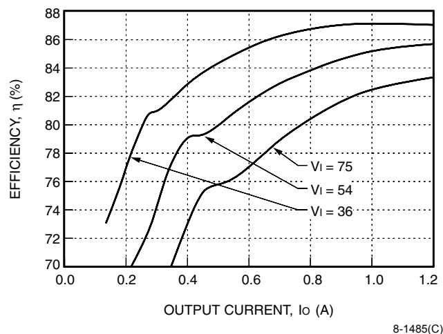
Figure 7. LW020C Typical Converter Efficiency vs. Output Current, T_A = 25^\circ\text{C}
