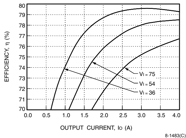
Figure 4. LW020F Typical Converter Efficiency vs. Output Current, T_A = 25\text{ }^{\circ}\text{C}
