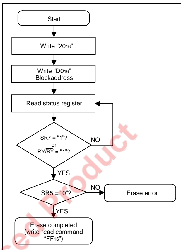
Fig 70. Erase flowchart
