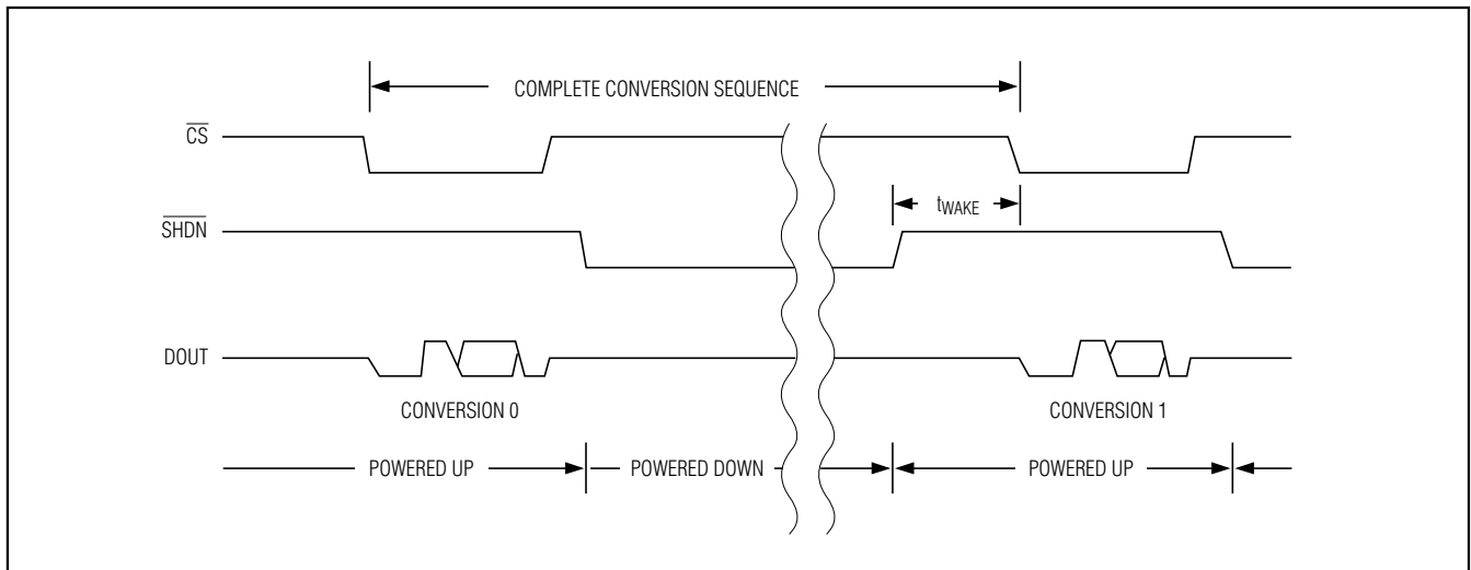
Figure 5. Shutdown Sequence
