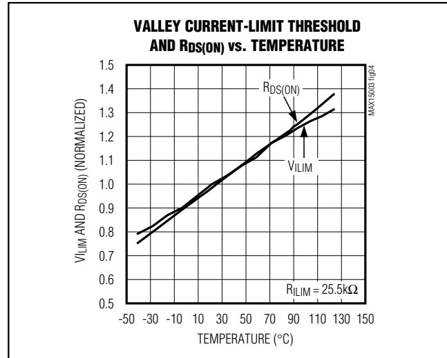
Figure 4. Current-Limit Trip Point and V_{\text{RDS(ON)}} vs. Temperature
