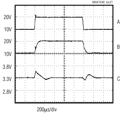
A. INPUT ( V_{IN} ), 10V/div B. LDIN (10V TO 20V), 10V/div C. LDOUT (3.3V), 500mV/div 20mA LOAD
