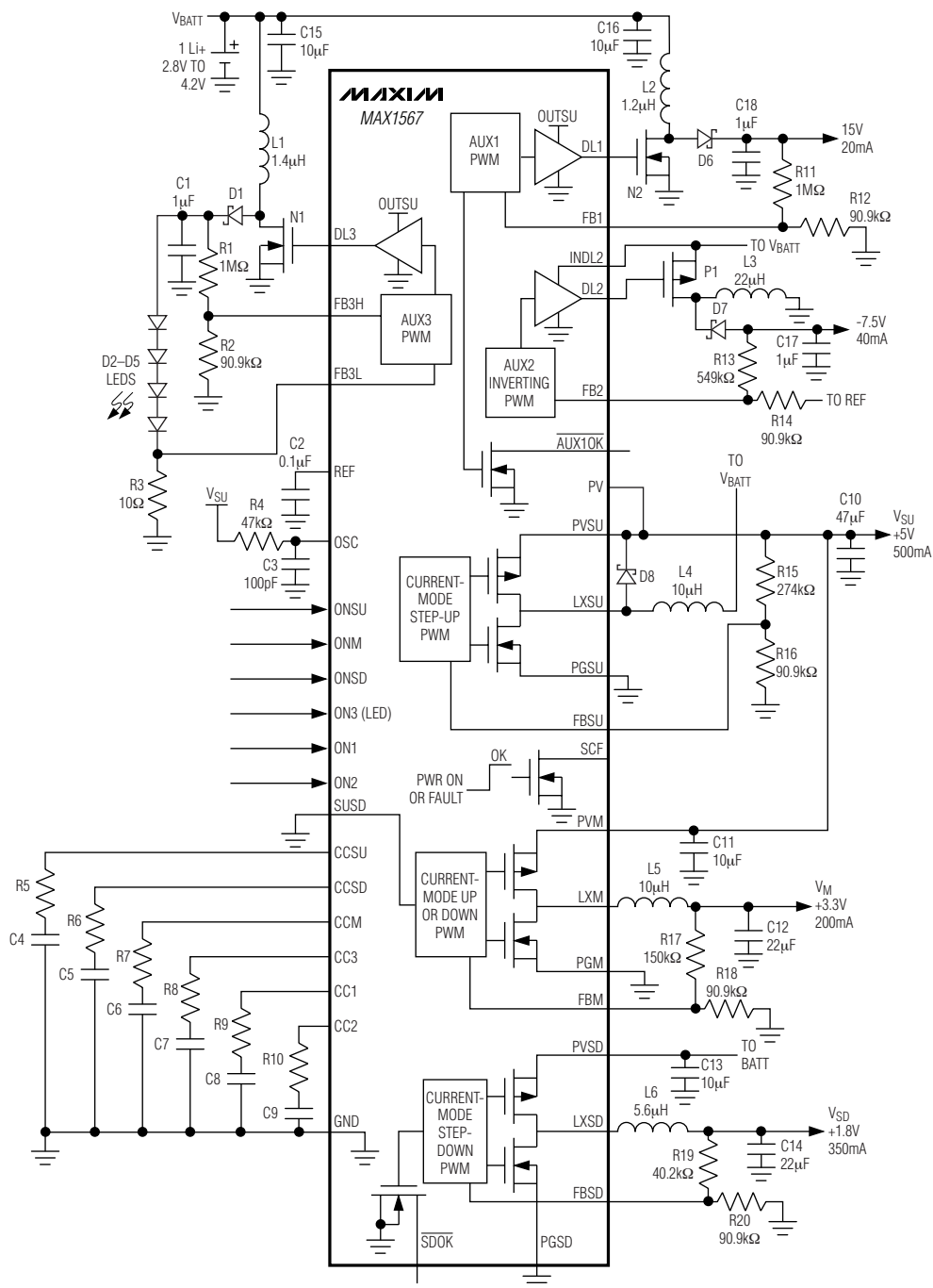
Figure 1. Typical 1-Cell Li+ Powered System (3.3V logic is stepped down from +5V, and 1.8V core is stepped down directly from the battery. Alternate connections are shown in the following figures.)
