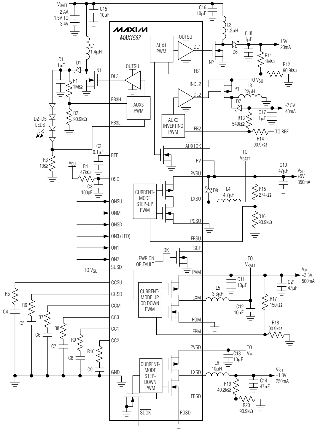
Figure 2. Typical 2-Cell AA-Powered System (3.3V is boosted from the battery and 1.8V is stepped down from V M (3.3V).)
