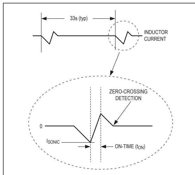
Figure 3. Ultrasonic Waveform
