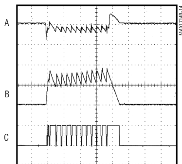
LOAD-TRANSIENT RESPONSE (8A COMPONENTS, V_{OUT} = 1.6V , 300kHz)
