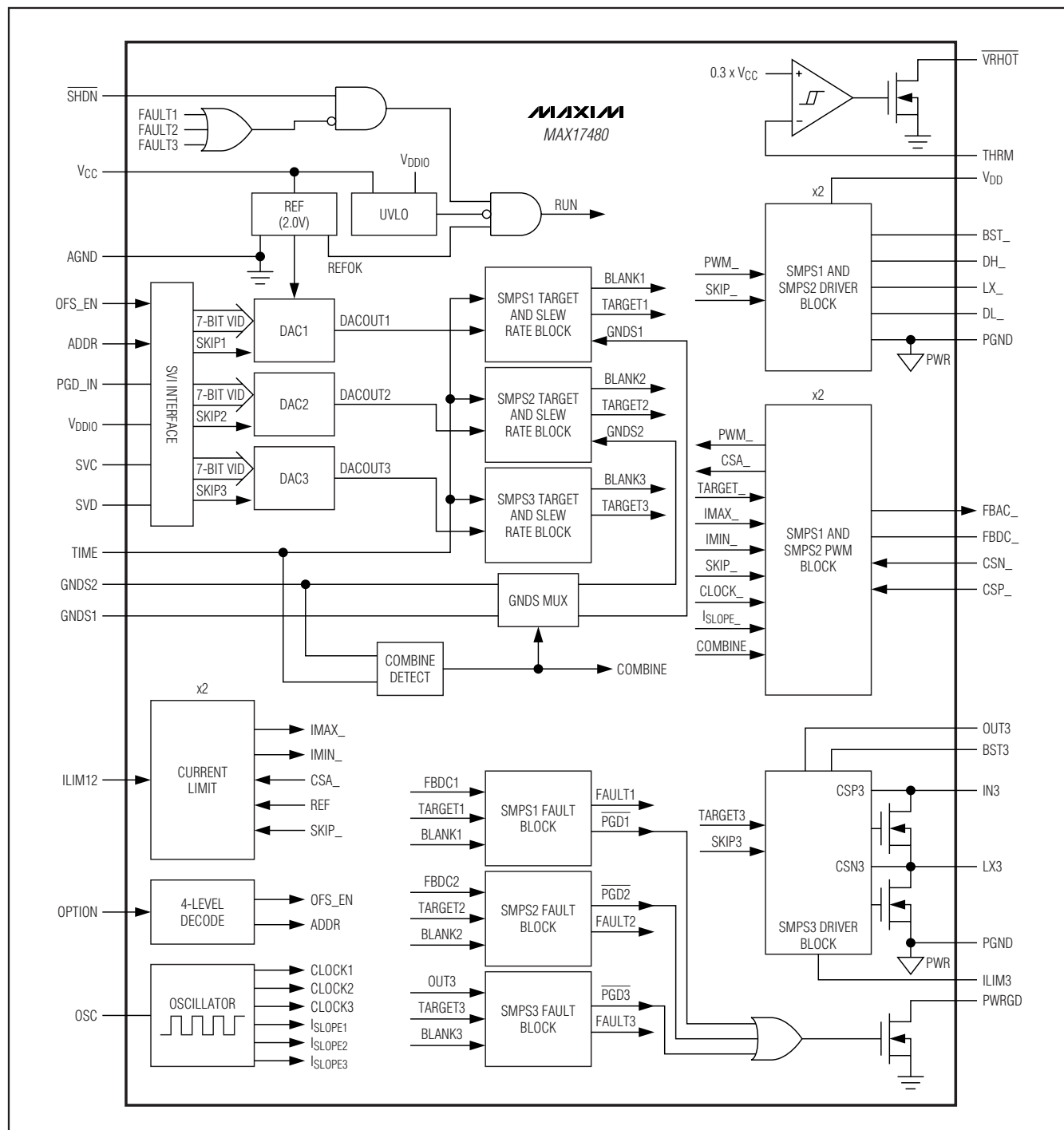
Figure 4. Functional Diagram
