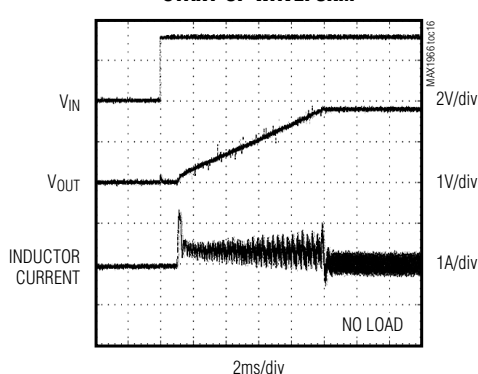
START-UP WAVEFORM
