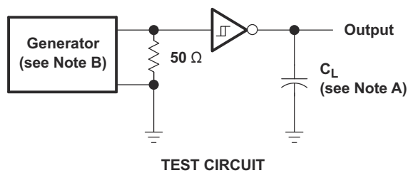
Figure 7-2. Driver Pulse Skew
