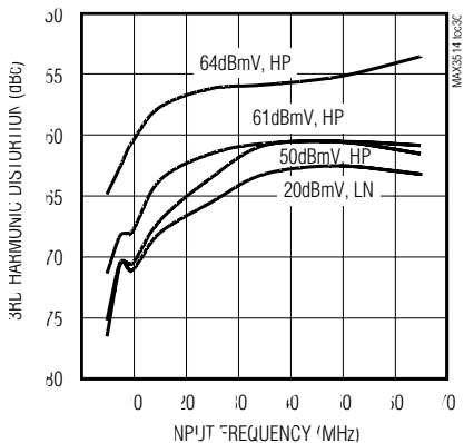
3RD HARMONIC DISTORTION vs. NPUT FREQUENCY, V_{CC} = 7.0V
