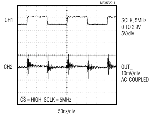
CLOCK FEEDTHROUGH
