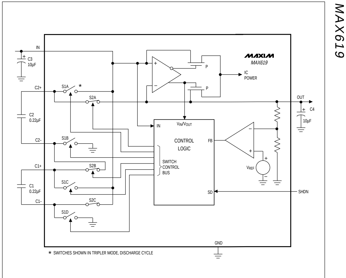
Figure 1. Block Diagram
