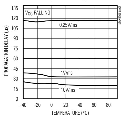
V_{\text{CC}} TO RESET PROPAGATION DELAY vs. TEMPERATURE
