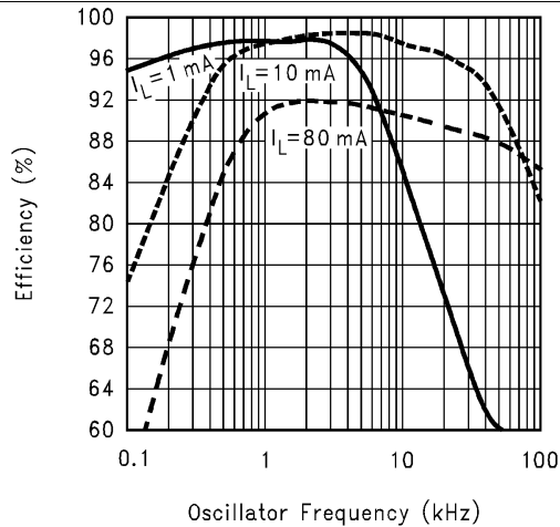
Figure 7. Efficiency vs Oscillator Frequency
