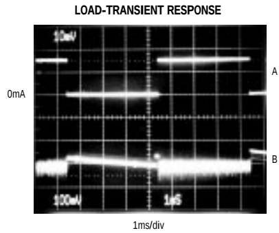
A: OUTPUT CURRENT, 20mA/div, I_{OUT} = 0\text{mA} to 30\text{mA} B: OUTPUT VOLTAGE RIPPLE, 100mV/div, V_{CC} = 5.0\text{V}
