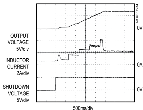
EXITING SHUTDOWN
