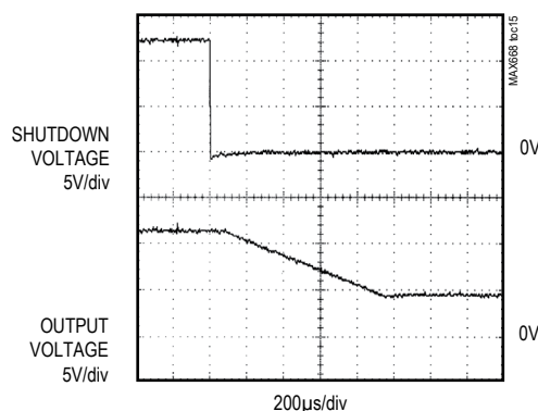
ENTERING SHUTDOWN
