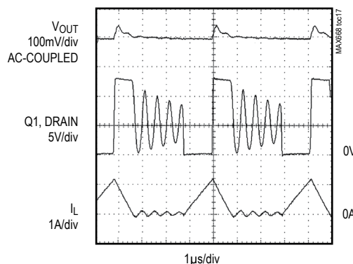
LIGHT-LOAD SWITCHING WAVEFORM
