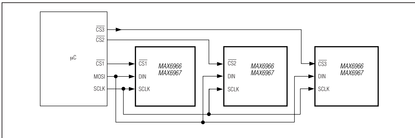
Figure 8. MAX6966/MAX6967 Multiple \overline{\text{CS}} Connection
