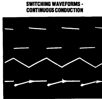
A = Switch Voltage (LX) 5V/div (4.8V to -5.3V) B = Inductor Current, 500mA/div C = Output Voltage Ripple, 50mV/div TIME = 2µs/div CIRCUIT OF FIG. 1 V IN = +5V T A = +25°C
