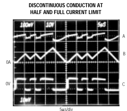
CIRCUIT OF FIGURE 2, V+ = 5V, VOUT = -5V, ILOAD = 140mA A: OUTPUT RIPPLE, 100mV/div B: INDUCTOR CURRENT, 500mA/div C: LX WAVEFORM, 10V/div
