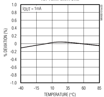
MAX8510 OUTPUT VOLTAGE ACCURACY vs. TEMPERATURE
