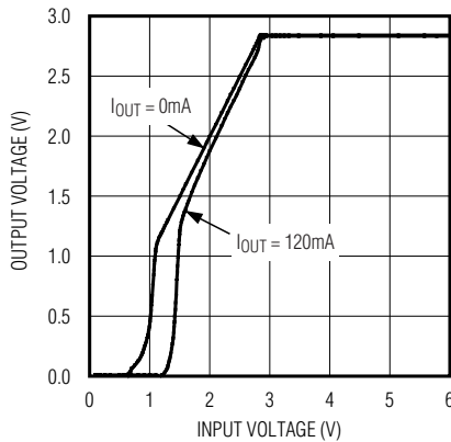
MAX8510 OUTPUT VOLTAGE vs. INPUT VOLTAGE
