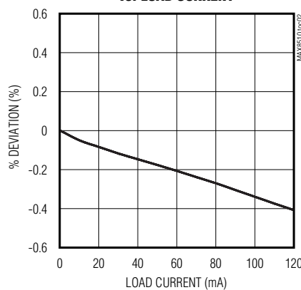
MAX8510 OUTPUT VOLTAGE ACCURACY vs. LOAD CURRENT
