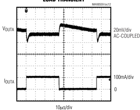
LOAD TRANSIENT
