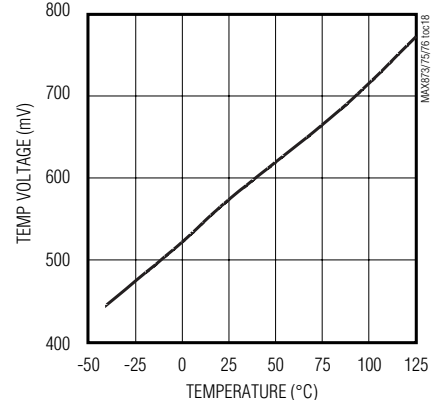
TEMP VOLTAGE vs. TEMPERATURE ( V_{OUT} = 2.5V )
