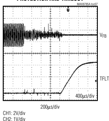
SECONDARY SHORT-CIRCUIT PROTECTION AND TIMEOUT
