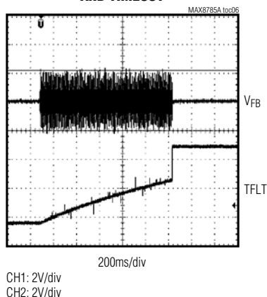
LAMP-OUT VOLTAGE LIMITING AND TIMEOUT
