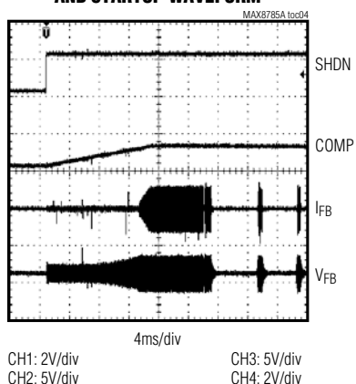
MINIMUM BRIGHTNESS OPERATION AND STARTUP WAVEFORM
