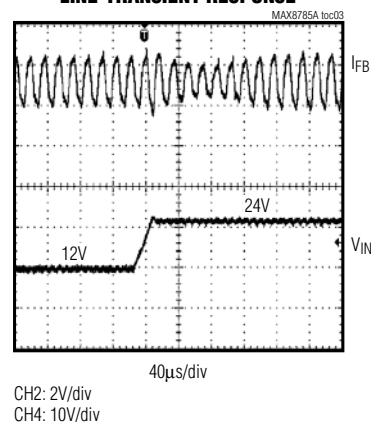
LINE-TRANSIENT RESPONSE
