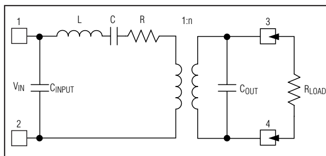
Figure 4. Electrical Model of Piezoelectric Transformer
