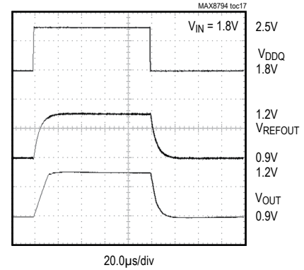
DYNAMIC OUTPUT-VOLTAGE TRANSIENT
