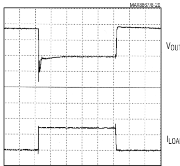
LOAD-TRANSIENT RESPONSE NEAR DROPOUT
