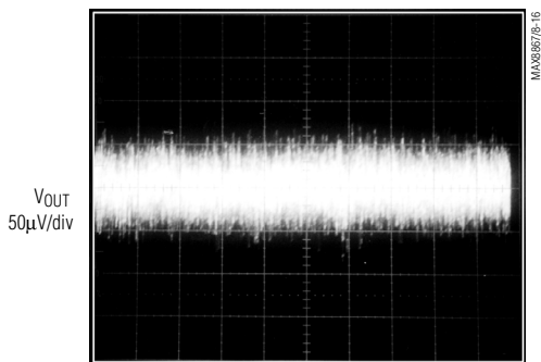
MAX886 E_K25 10Hz TO 100kHz OUTPUT NOISE
