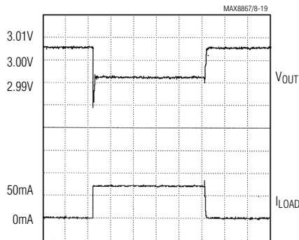
LOAD-TRANSIENT RESPONSE
