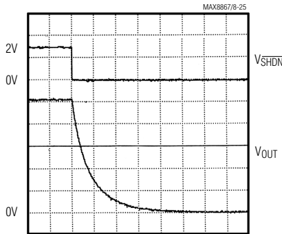
MAX8868 ENTERING SHUTDOWN
