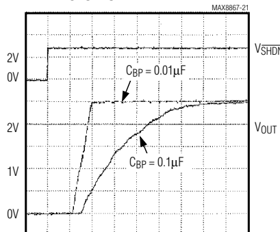
MAX886 E_K25 SHUTDOWN EXIT DELAY
