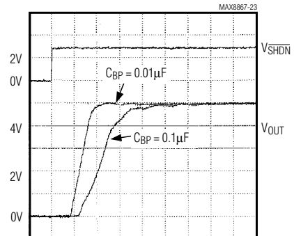
MAX886 E_K50 SHUTDOWN EXIT DELAY
