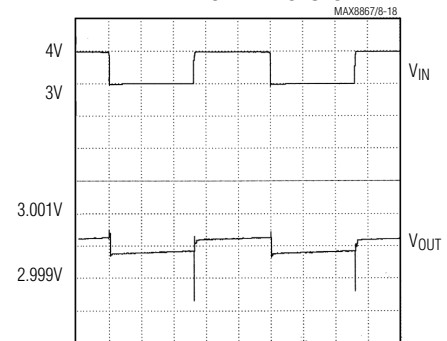
LINE-TRANSIENT RESPONSE
