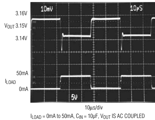
LOAD-TRANSIENT RESPONSE
