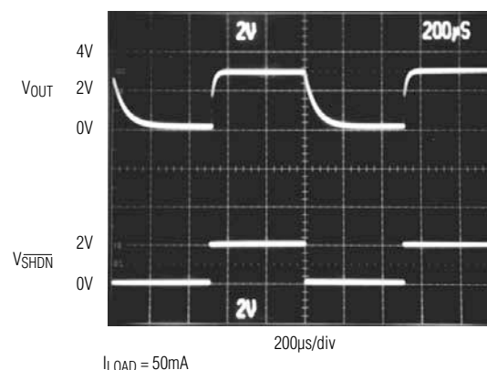
MAX8874 SHUTDOWN
