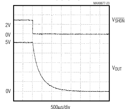
MAX8878, NO LOAD
