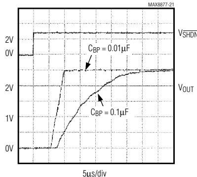
MAX8877_EUK25, I_{LOAD} = 50mA
