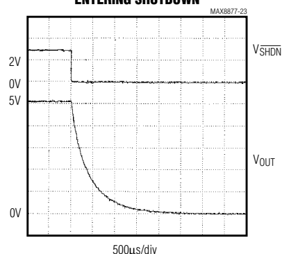
ENTERING SHUTDOWN
