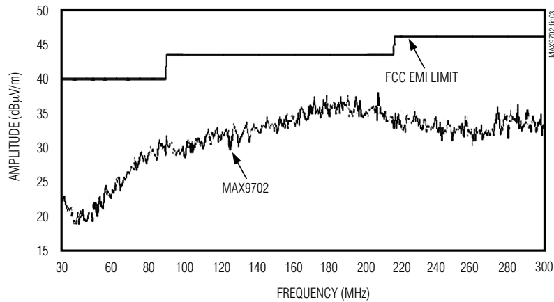
Figure 3. MAX9702 EMI with 76mm of Speaker Cable
