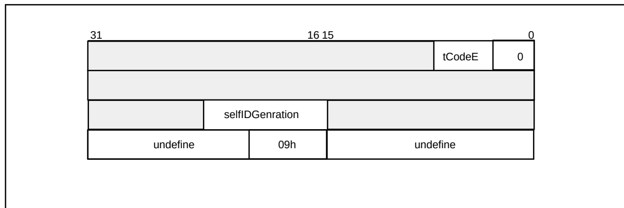
Fig. 5.1 Bus Reset Packet Format
