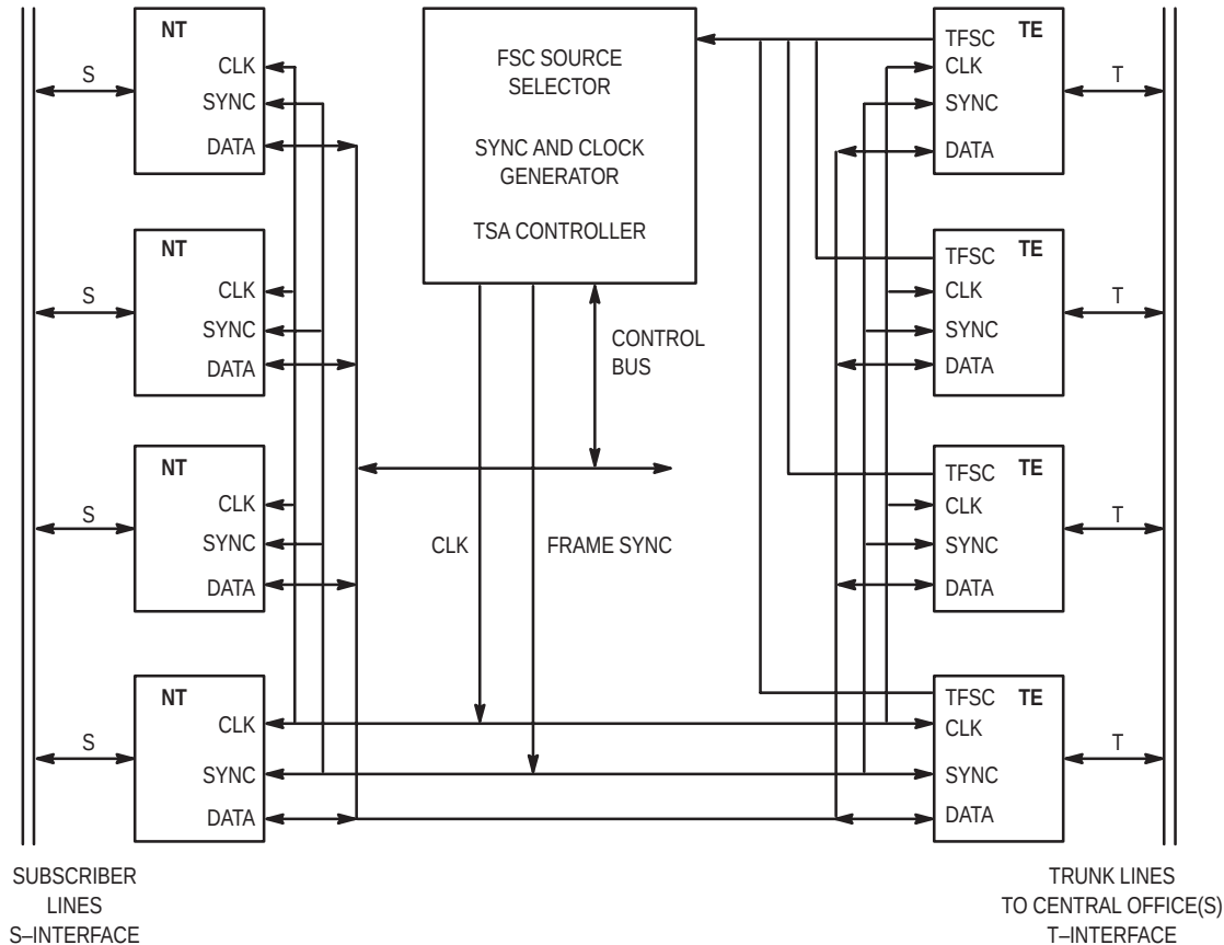
Figure 13–3. NT2 Architecture
