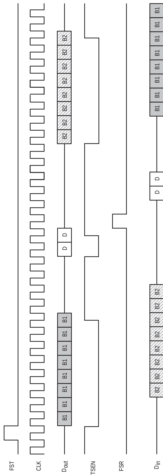
Figure 4–8. Timeslot Operation with Independent Slave Frame Syncs, \overline{\text{TSEN}}
