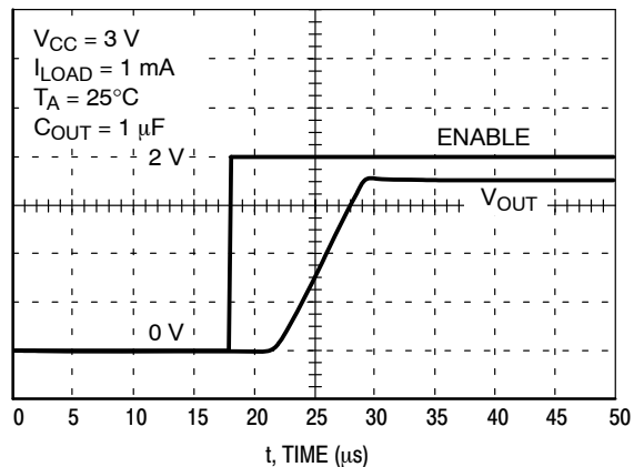
Figure 21. Enable Response
