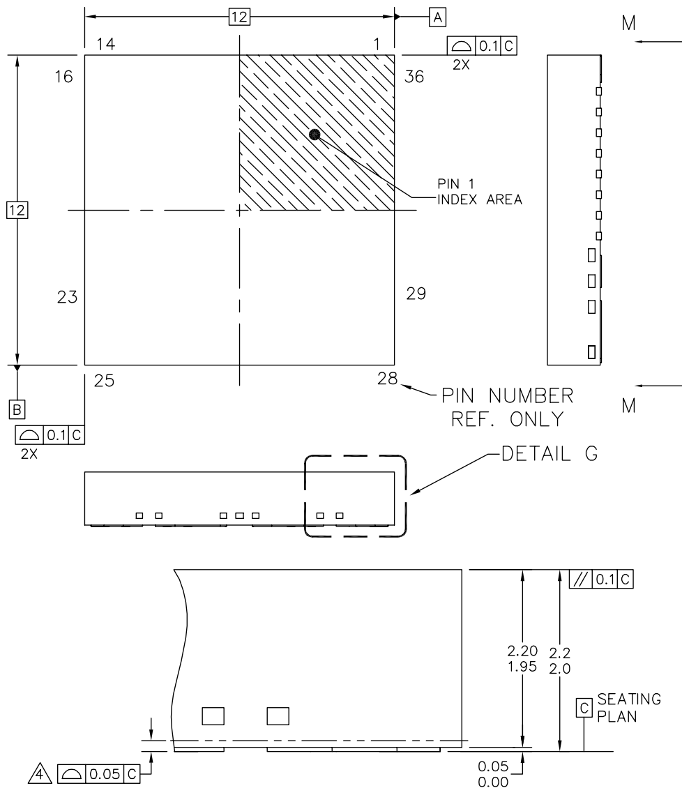
DETAIL G
