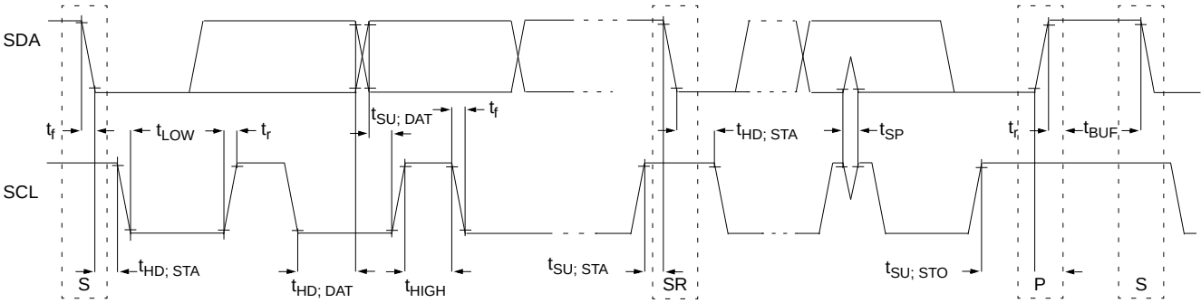
Figure 10-14 Timing Definition for Fast and Standard Mode Devices on the I²C Bus
